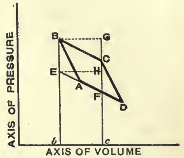
FIG. 5.—Elementary Carnot Cycle for Gas.
